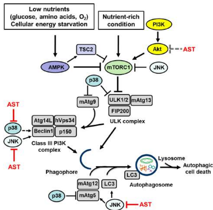
Figure 1. The signaling pathways that regulate autophagy and autophagy-related proteins that are affected by astaxanthin (AST). Low nutrients levels (glucose or amino acid withdrawal, oxygen deprivation) and cellular energy starvation activate AMPK, which inactivates mTORC1 via stimulation of TSC2. When mTORC1 is inactivated, dephosphorylated ULK1/2 and mAtg13 form a stable ULK complex (ULK1/2-mAtg13-FIP200 complex). The ULK complex is the regulator of the autophagy pathway that initiates organization of the phagophore membranes. Upon induction of autophagy, mAtg9, a major transport protein, transports membrane lipids from donor organelles to the phagophore. Two ubiquitin-like protein conjugation systems, mAtg12 along with its conjugate mAtg5 and LC3 play roles in elongation and expansion of the phagophore to induce autophagosome formation and closure. In the Class III PI3K complex, hVsp34 works in concert with its regulatory adaptor proteins p150 and Beclin 1 to regulate vesicular trafficking and vacuolar protein sorting. p150 is required for association of hVsp34 with the phagophore membrane. Binding of Beclin 1 to Atg14L directs the class III PI3K complex to the phagophore, where it initiates both recruitment of the Atg machinery and phagophore nucleation. Under nutrient-rich conditions, mTOR signaling is activated. Activated mTORC1 induces phosphorylation of mAtg13 and dissociation of the ULK complex leading to inhibition of autophagy. PI3K/Akt activates the mTOR pathway leading to inhibition of autophagy. JNK inhibits the mTOR pathway and increases expression of Beclin 1, mAtg5, and LC3, resulting in induction of autophagy. p38 increases expression of Beclin 1 and induces autophagy. In contrast, p38 phosphorylates ULK1 and blocks ULK1 activation of its downstream effector mAtg13. Also, p38 inhibits starvation-induced autophagy by phosphorylating mAtg5 and blocking autophagosome fusion with lysosomes. p38 alters trafficking of mAtg9 and autophagosome formation. In the context of autophagy, LC3 is involved in elongation and expansion of the phagophore to induce autophagosome formation and closure. mAtg12 along with its conjugate mAtg5 and LC3 play roles in this process. In relation to Akt signaling, AST inhibits the activation of Akt, leading to induction of autophagy via the Akt/mTOR pathway and increases expression of Beclin 1 and LC3. AST blocks JNK and reduces the levels of the autophagy-related proteins Beclin 1 and LC3. AST inhibits p38 and JNK and, consequently, it reduces autophagy by modulating MAPK-mediated release of Beclin 1. Dotted lines represent autophagy activation by astaxanthin (by inhibiting Akt activation) or p38 (by increasing Beclin 1 level).
